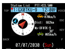
Own station/ other station relative display: Shows the position of own station, and relative distance, direction, heading, and speed of other stations
