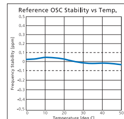
TCXO temperature drift characteristics
