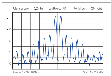
14 MHz transmit IMD example (100 W output)
